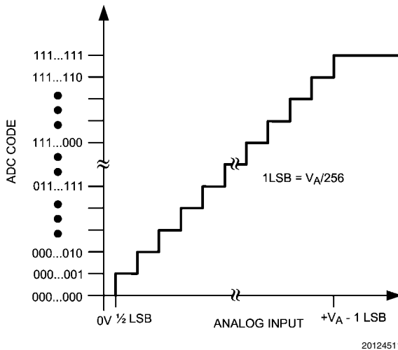
FIGURE 3. Ideal Transfer Characteristic
